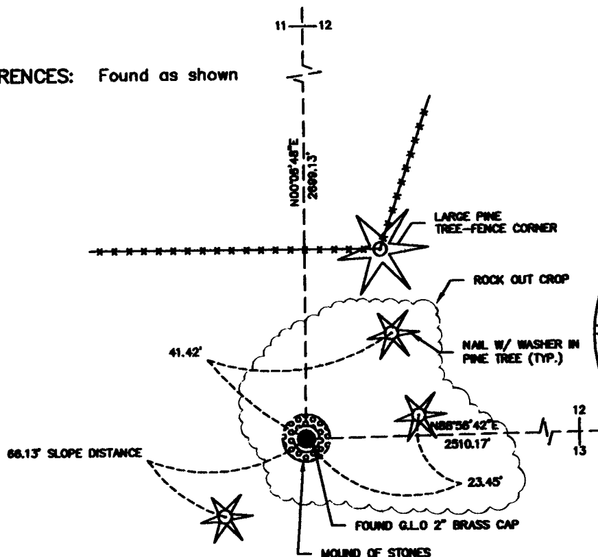
FOUND MONUMENT DETAIL
